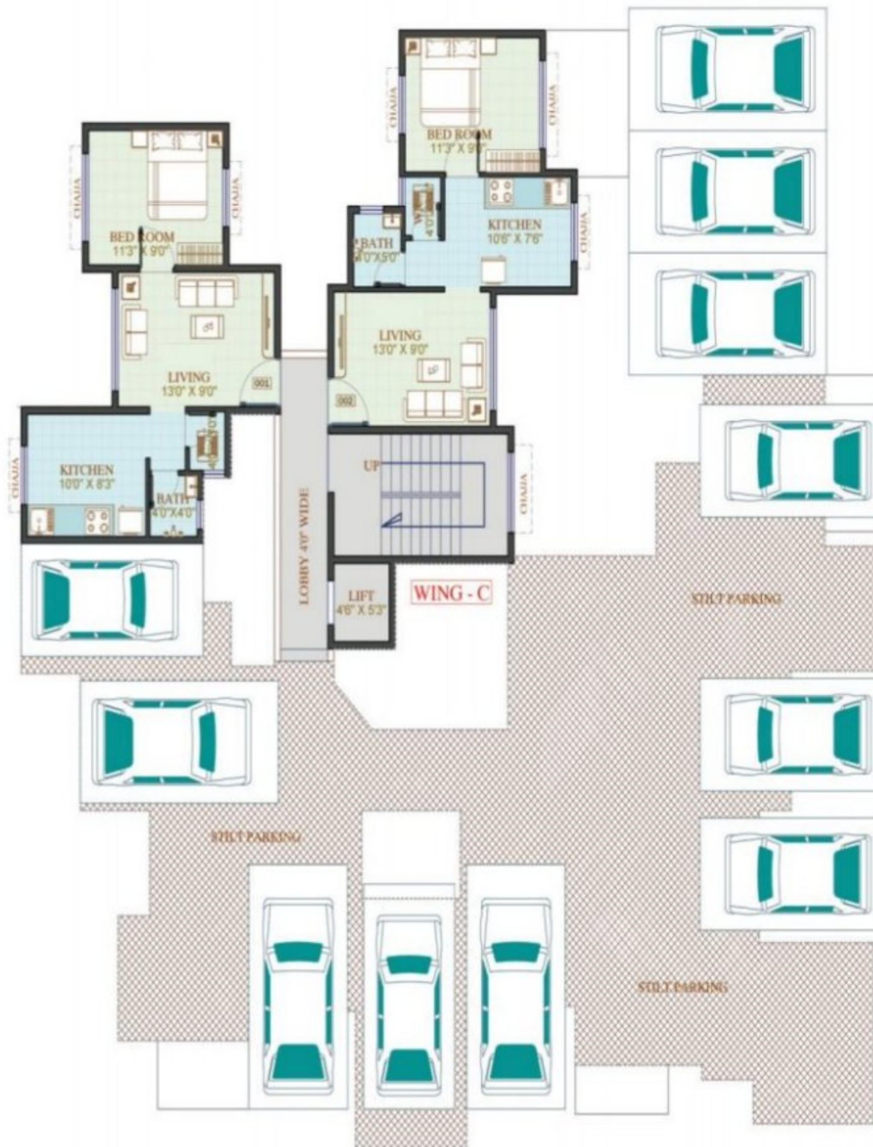
Wing C Ground Floor Plan
